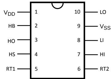
Figure 1. 10-Lead VSSOP, WSON
